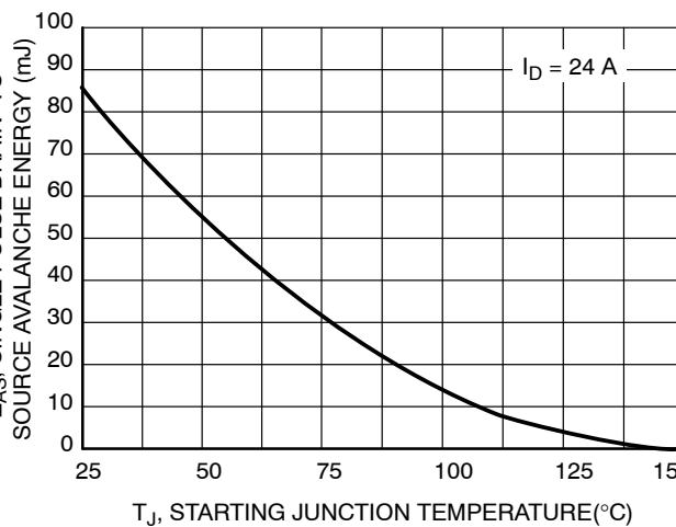
Figure 12. Maximum Avalanche Energy vs. Starting Junction Temperature
