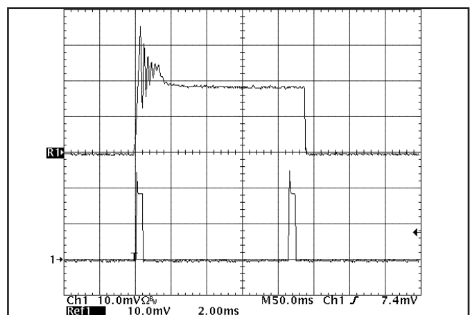
Figure 18: Load current ( 10\text{A}/\text{div} ) as a function of time when the converter attempts to turn on into a 10\ \text{m}\Omega short circuit. Top trace ( 2.0\text{ms}/\text{div} ) is an expansion of the on-time portion of the bottom trace.
