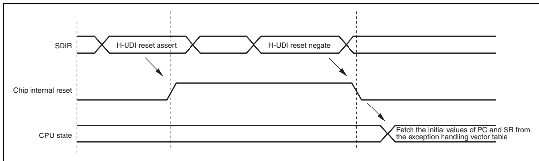
Figure 33.4 H-UDI Reset
