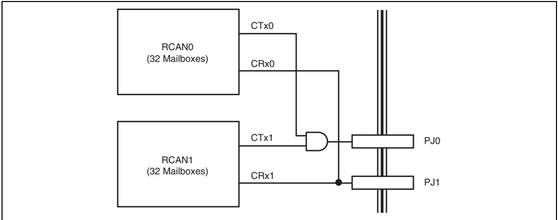
Figure 19.30 Connection Example when Using RCAN-TL1 as 1-Channel Module (64 Mailboxes × 1 Channel)
