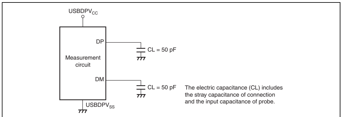
Figure 35.75 Measurement Circuit (Full-Speed)
