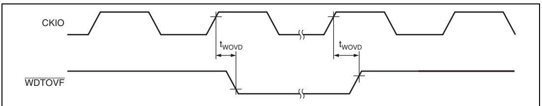
Figure 35.50 WDT Timing
