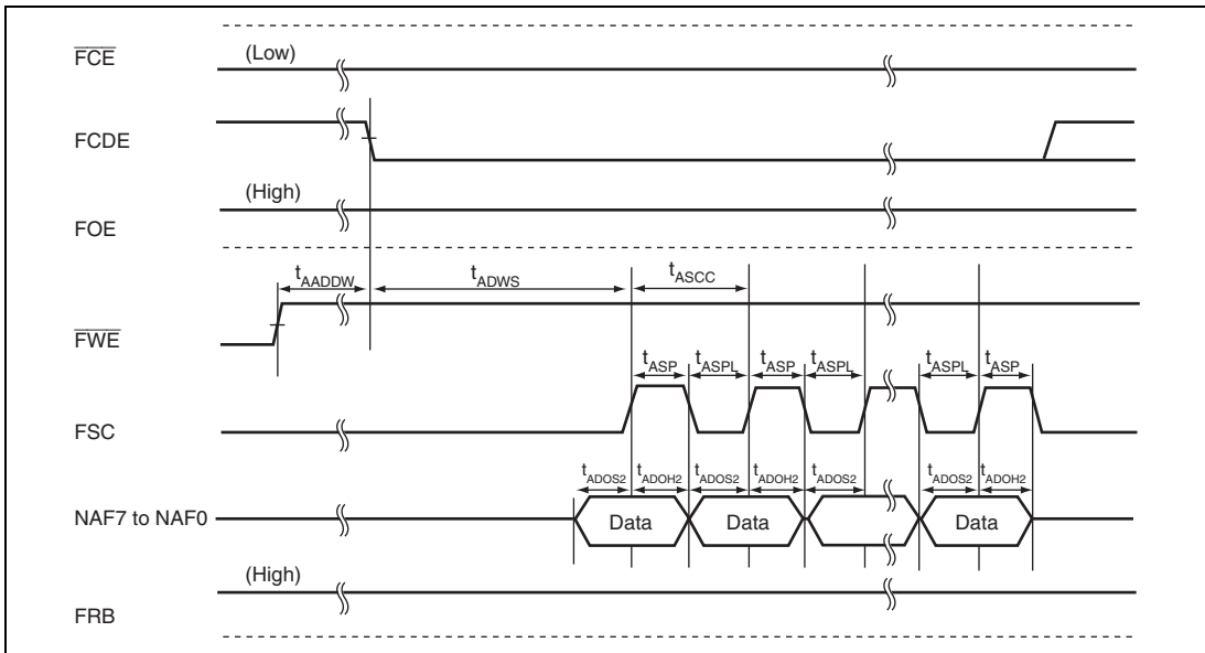
Figure 35.67 AND Type Flash Memory Data Write Timing
