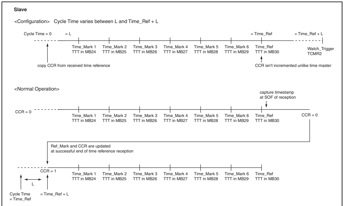
Figure 19.20 Time Slave
