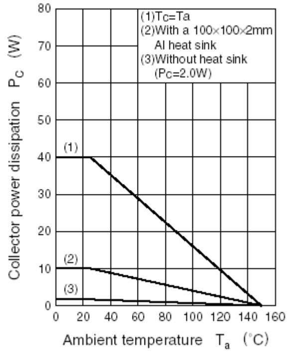
Fig.8 Power Derating
