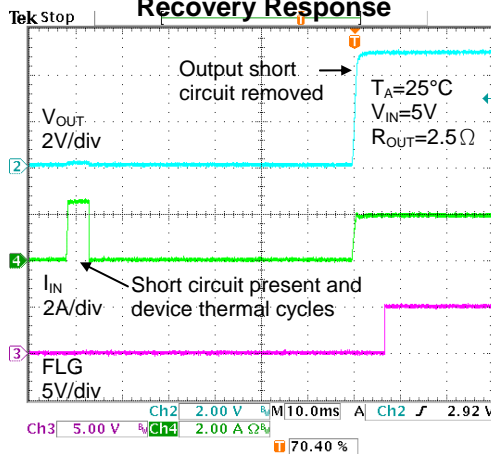
Short-Circuit to Full-Load Recovery Response
