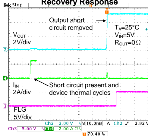
Short-Circuit to No-Load Recovery Response
