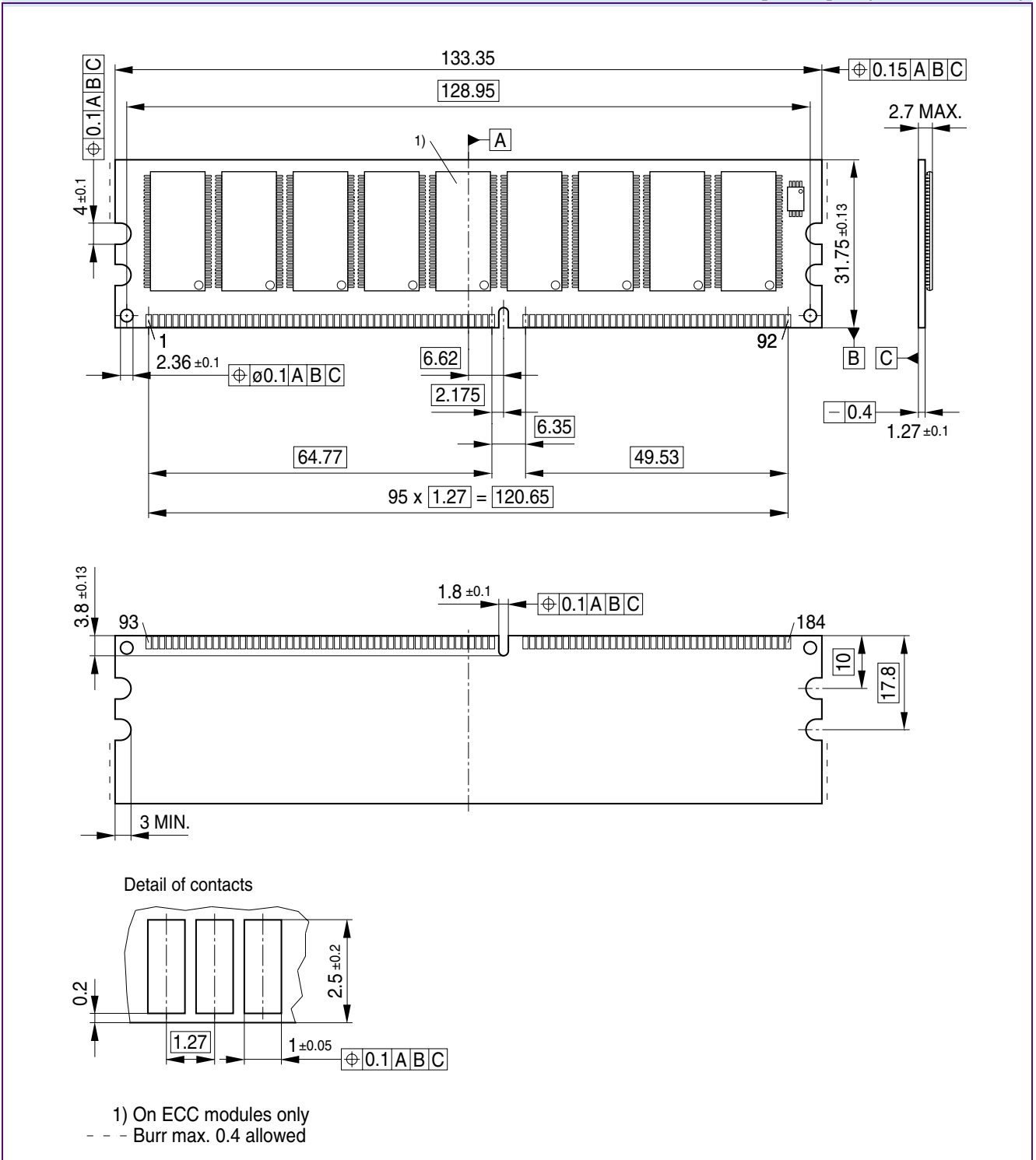
FIGURE 4 Raw Card A DDR UDIMM HYS72D64300HU-[5/6/7F]-B (1 Rank Module)
