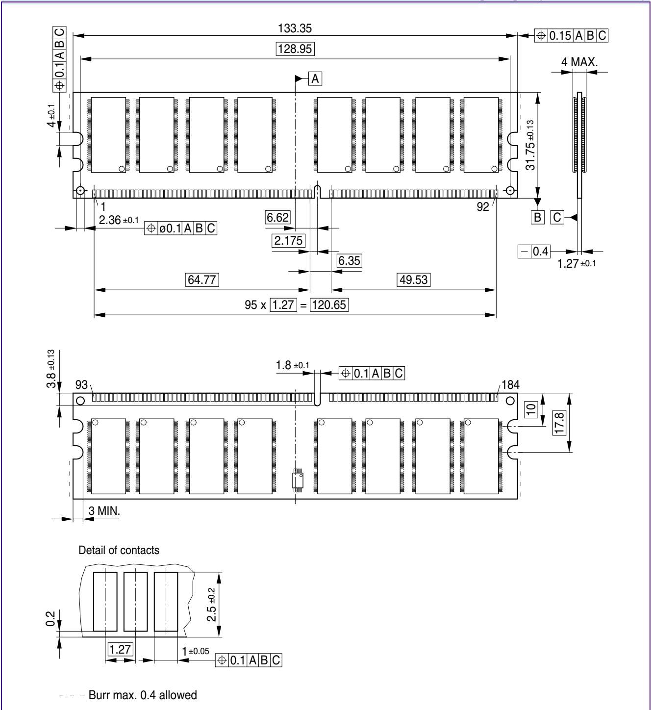
FIGURE 5 Raw Card B DDR UDIMM HYS64D128320HU-[5/6/7]-B (2 Ranks Module)
