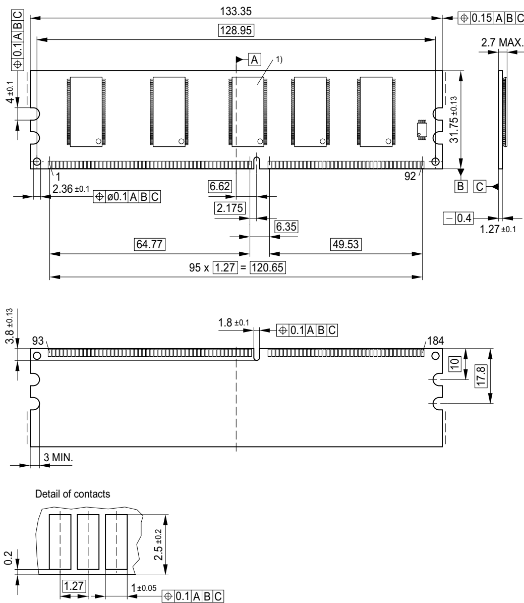
Raw Card C DDR UDIMM HYS64D32301HU-5-B (1 Rank Module)
