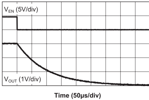
Turn-Off Response Time ( I = 100\text{mA} )
