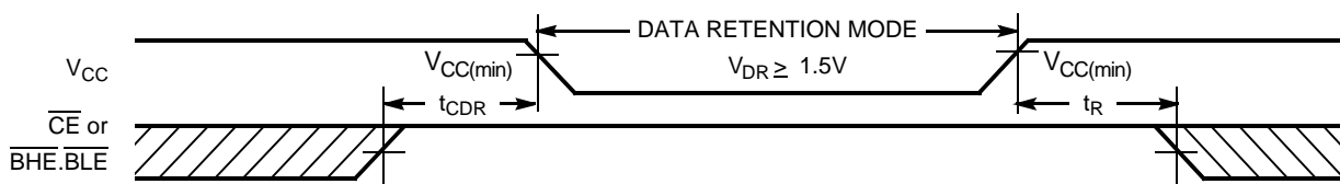
Figure 5. Data Retention Waveform [1, 11]
