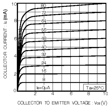
Ground emitter output characteristics
