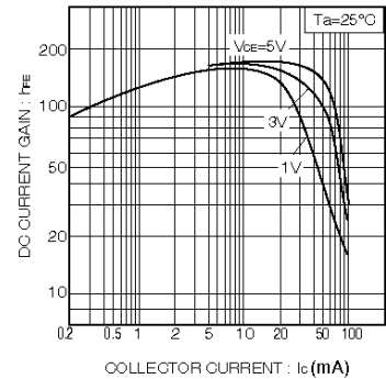
DC current gain vs. collector current (I)
