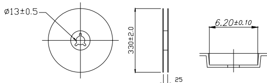
REEL DIMENSION
