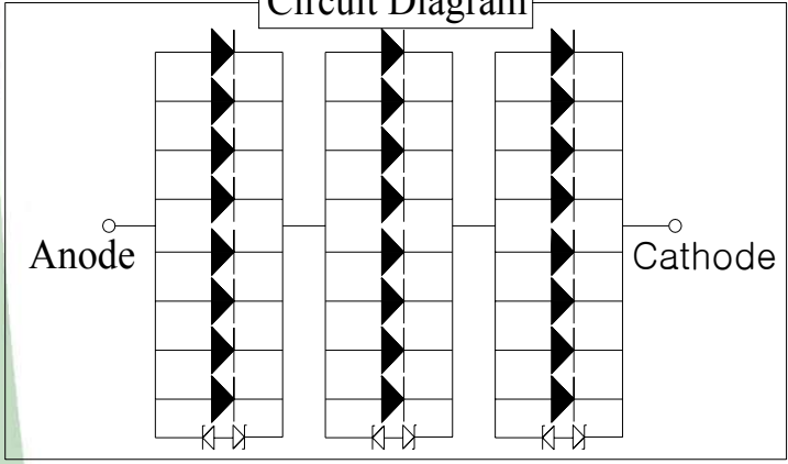
Circuit Diagram
