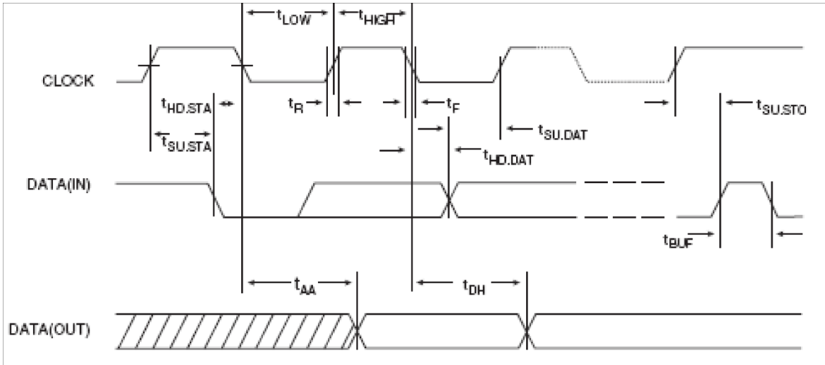
Figure 9-1. AT69170E serial data transfer - TWI
