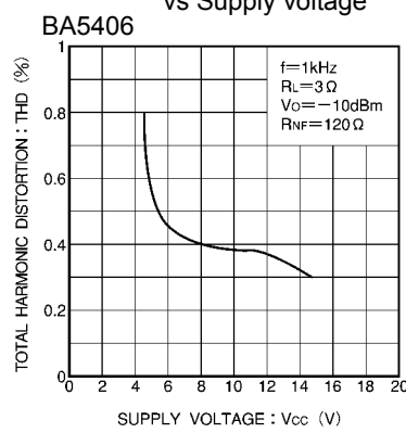
Fig.12 Distortion vs power supply voltage
