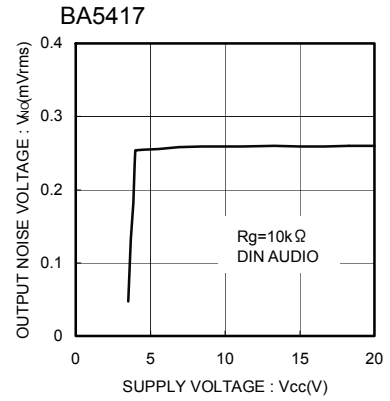
Fig.22 Output noise voltage vs Supply voltage
