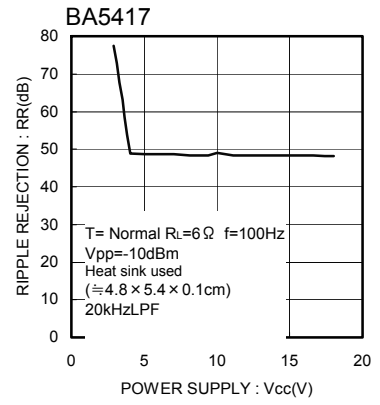
Fig.33 Ripple rejection ratio vs. Supply Voltage
