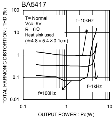
Fig.32 Total harmonic distortion vs. Output power
