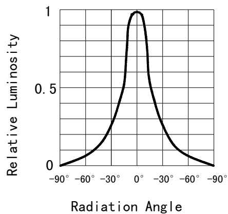
Fig 6. Relative Luminous Intensity vs. Radiation Angle
