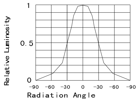
Fig 6. Relative Luminous Intensity vs. Radiation Angle
