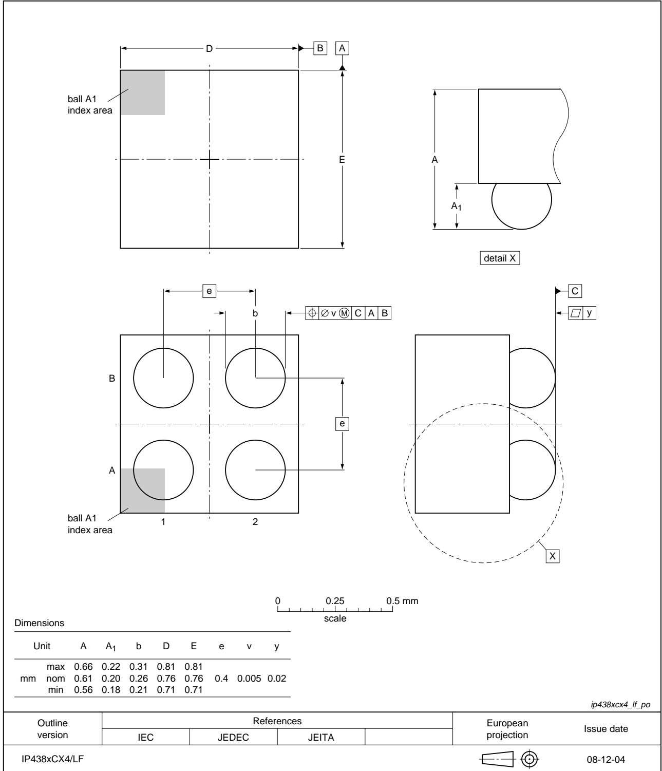
Fig 21. Package outline IP438xCX4/LF (WLCSP4)
