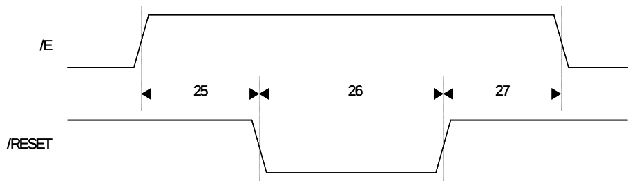
Figure 10: Reset Cycle
