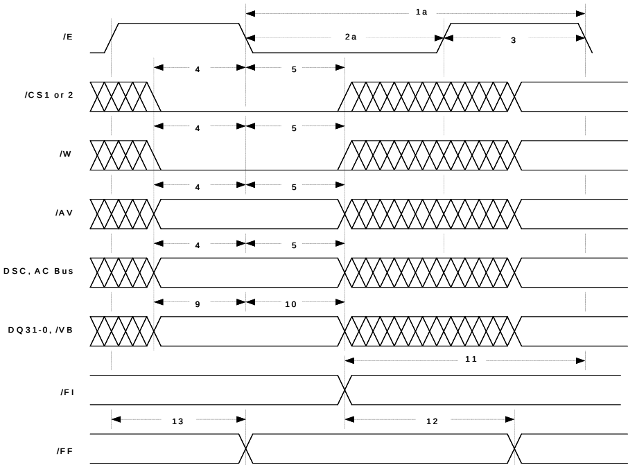
Figure 8: Write Cycle
