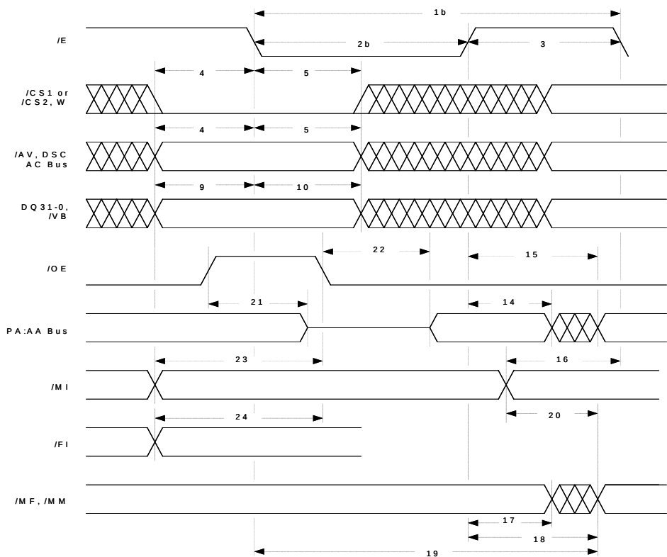
Figure 9: Compare Cycle
