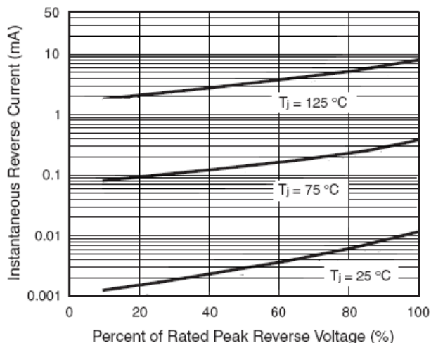
Figure 4. Typical Reverse Characteristics Per Diode
