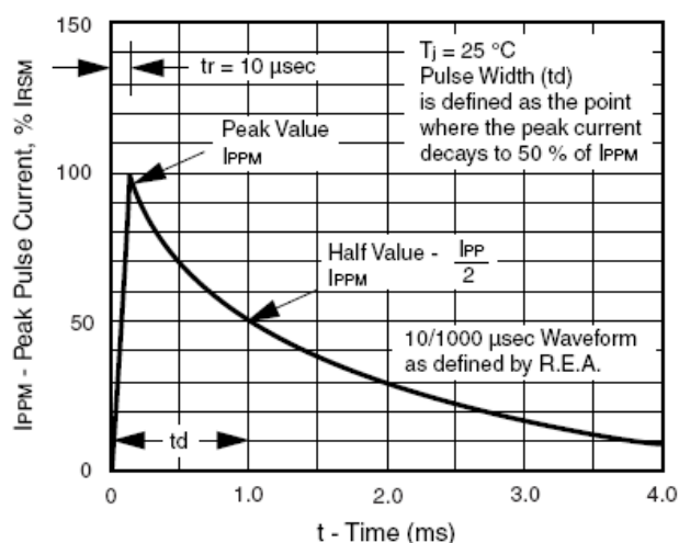
Figure 3. Pulse Waveform
