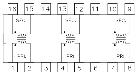
SCHEMATIC DIAGRAM
