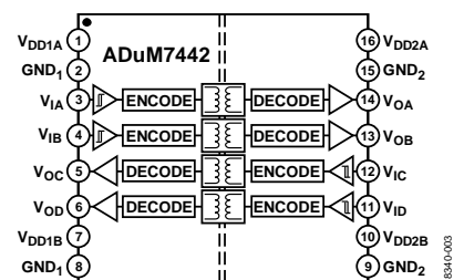
Figure 3. ADuM7442
