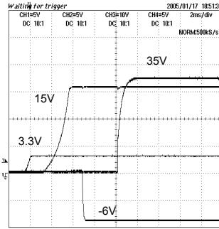
Fig.17 Start-up Sequence
