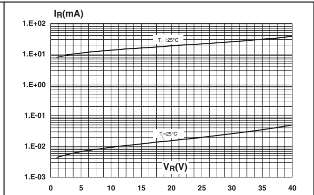
Figure 10. Reverse leakage current versus reverse voltage applied (typical values)
