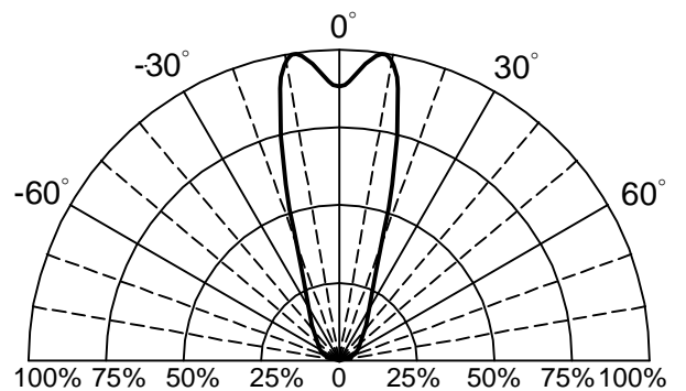
Fig.6 Directivity Radiation
