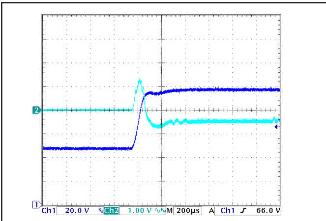
Figure 15: Output voltage response to step-change in input voltage ( 50\text{V} to 100\text{V} in 200\mu\text{s} ). Load cap: 470\mu\text{F} , 15\text{ m}\Omega ESR tantalum capacitor. Ch 1: V_{in} ( 20\text{V/div} ), Ch 2: V_{out} ( 1\text{V/div} ), at zero load current.
