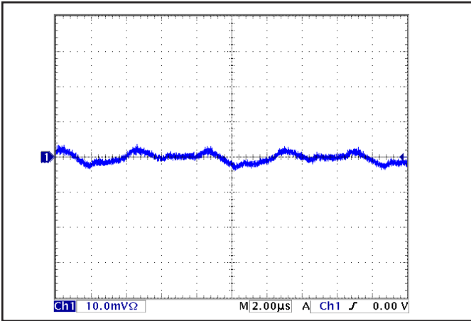
Figure 13: Input reflected ripple current, i_s , through a 4.7\mu\text{H} source inductor, using a 100\mu\text{F} input capacitor, at nominal input voltage and rated load current ( 10\text{mA/div} ). See Figure 11.
