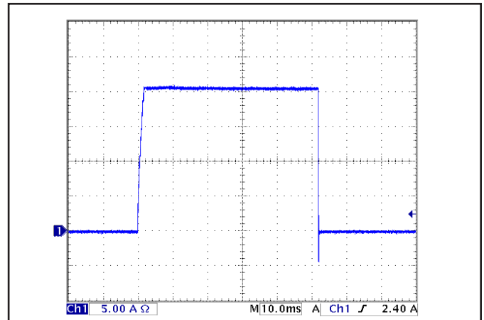
Figure 16: Load current ( 5\text{A/div} ) as a function of time when the converter attempts to turn on into a 10\text{ m}\Omega short circuit.
