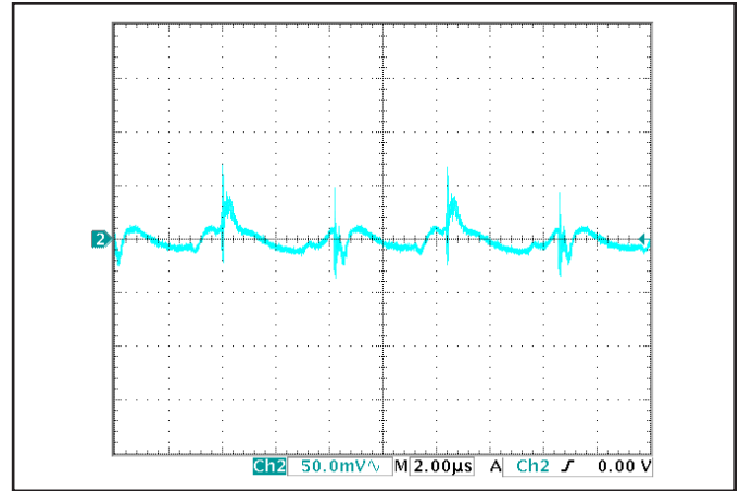
Figure 14: Output voltage ripple at nominal input voltage and rated load current ( 50\text{mV/div} ). Load capacitance: 1\mu\text{F} ceramic capacitor and 10\mu\text{F} tantalum capacitor. Bandwidth: 500 MHz. See Figure 11.
