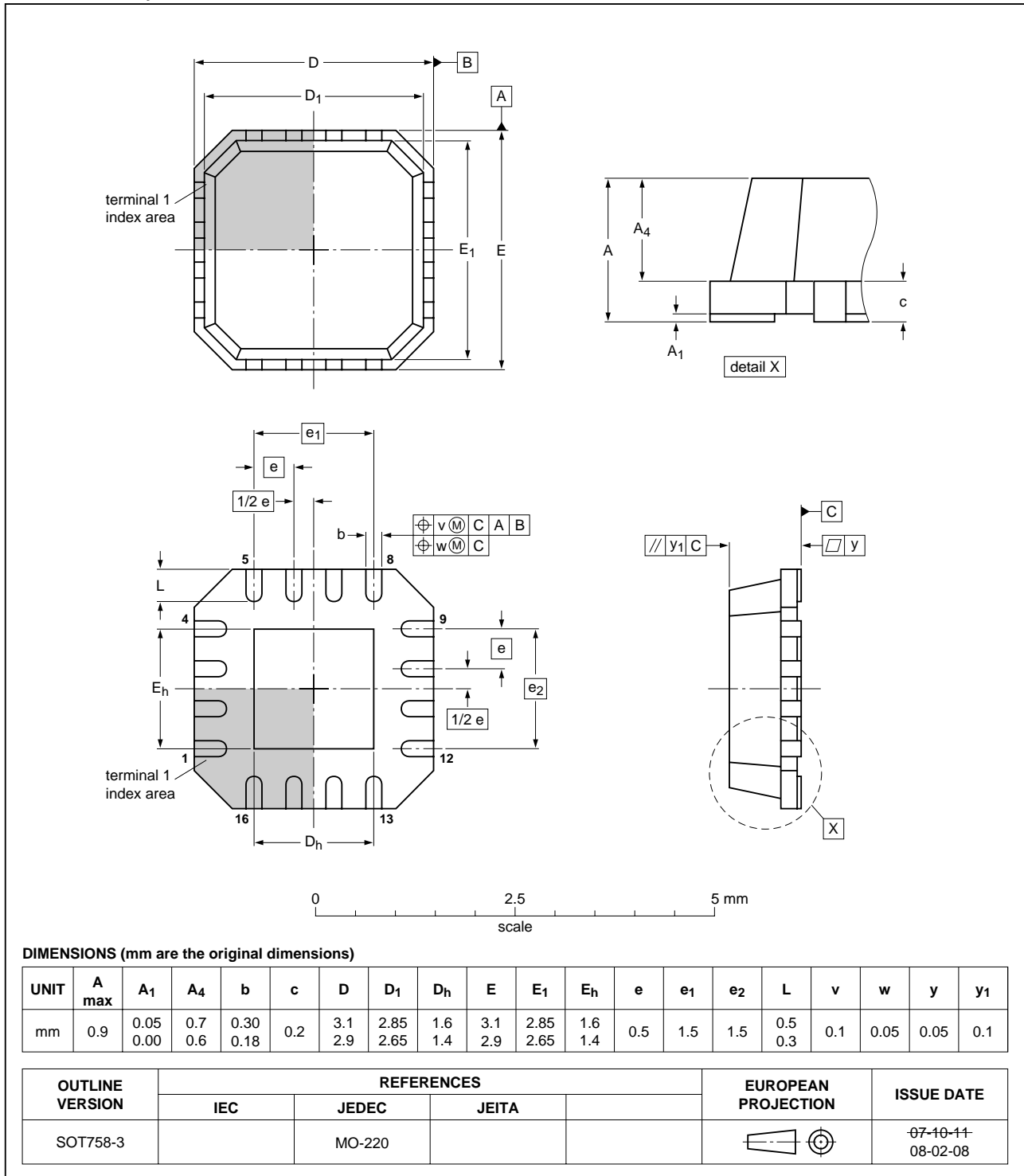
Fig 15. Package outline SOT758-3 (HVQFN16)
