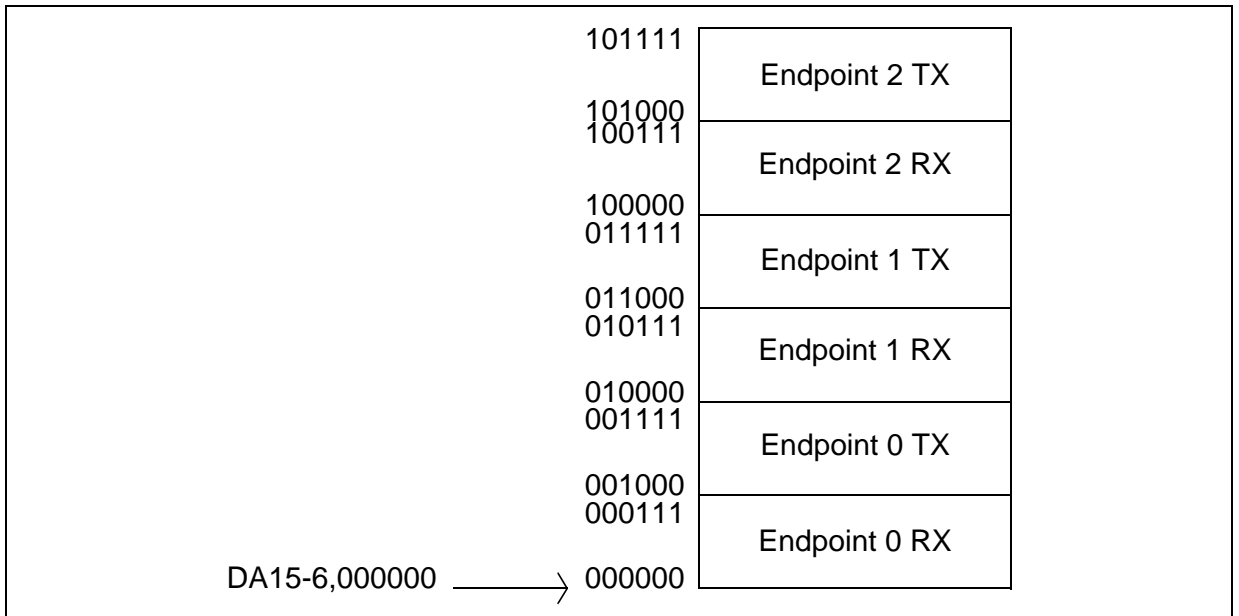
Figure 42. DMA buffers
