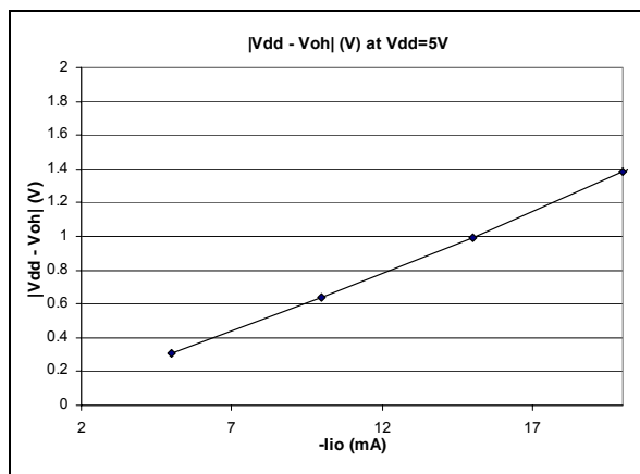
Figure 67. |V_{DD}-V_{OH}| @ V_{DD}=5 V (high current)
