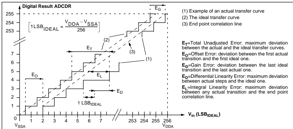
Figure 75. ADC accuracy characteristics
