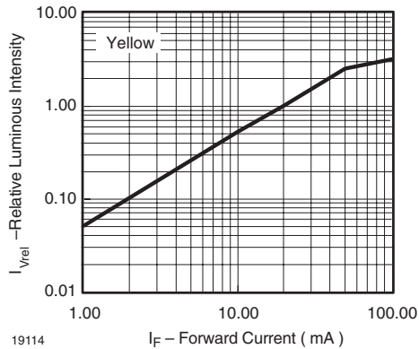
Figure 29. Relative Luminous Intensity vs. Forward Current
