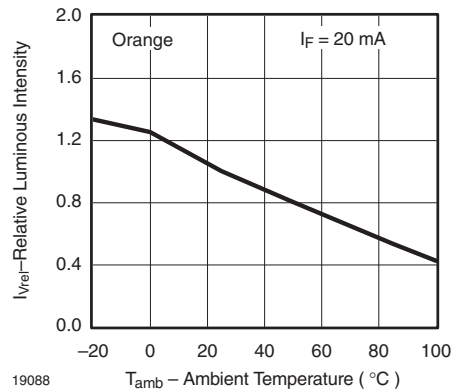
Figure 4. Relative Luminous Intensity vs. Amb. Temperature
