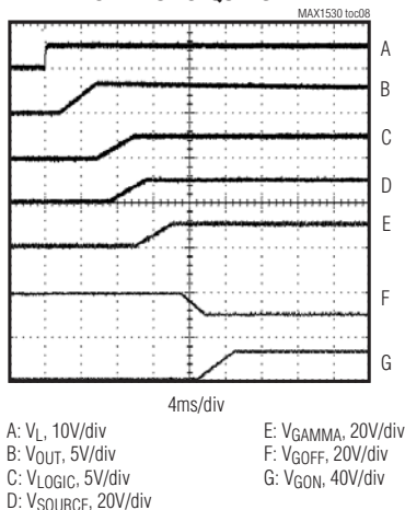
STARTUP SEQUENCE
