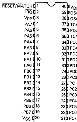
40-Pin Dual-In-Line Package
