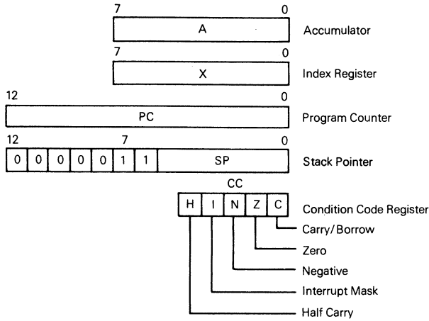
Figure 2-5. Programming Model
