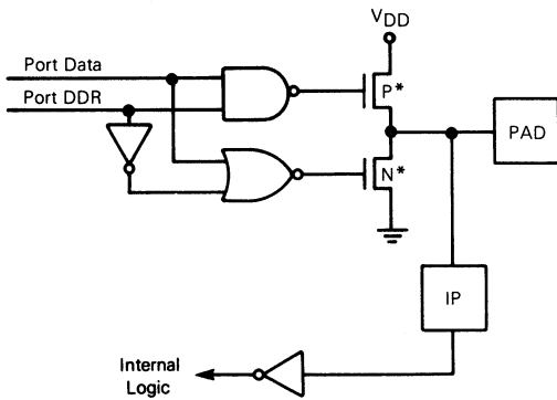
Figure 2-3. Parallel Port I/O Circuitry
