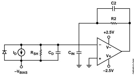
Figure 44. High Speed Photodiode Preamplifier
