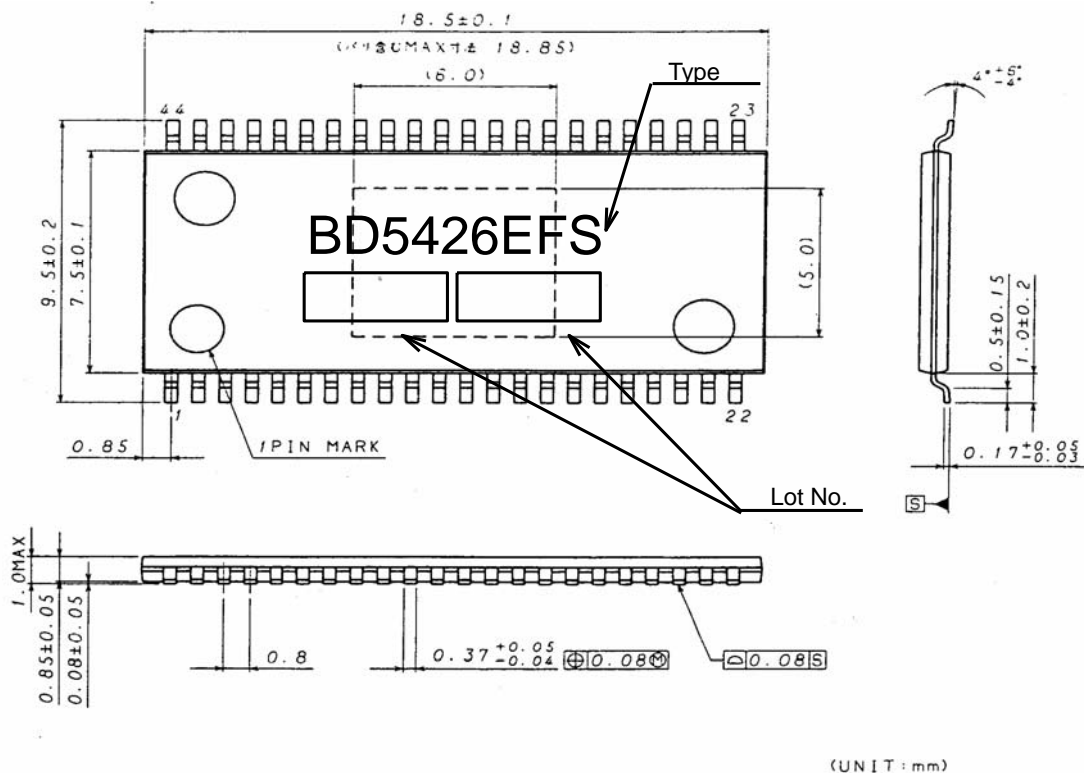
Fig. 24 Outer Dimensions and Inscriptions of HTSSOP-A44 Package
