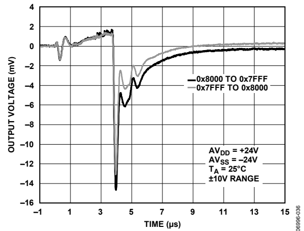
Figure 38. Digital-to-Analog Glitch
