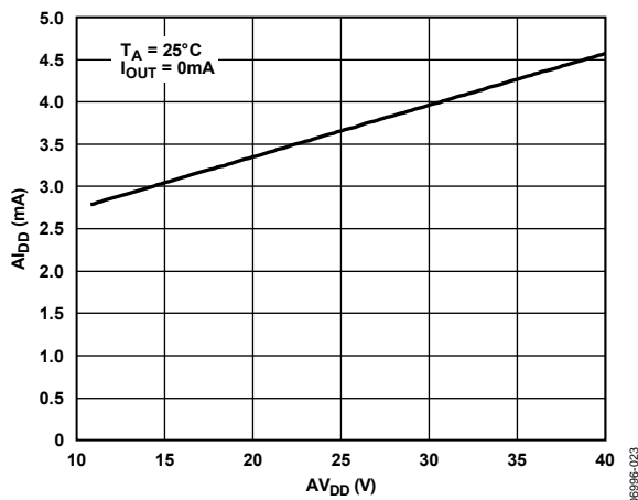
Figure 9. I_{1DD} vs. AV_{1DD}
