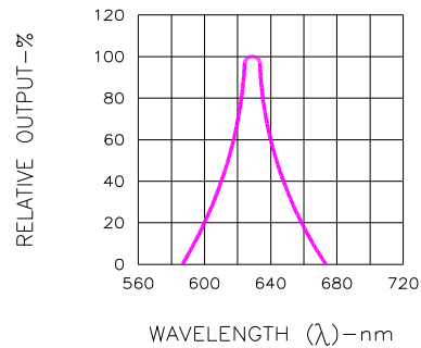
Fig.2 SPECTRAL RESPONSE
