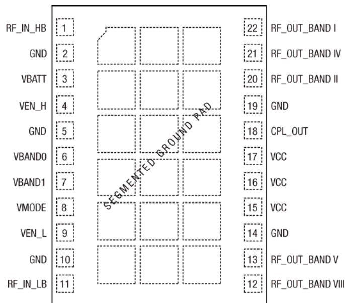
Figure 2. SKY77602 Pad Configuration
