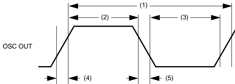
Figure 13-2. OSC Out Timing
