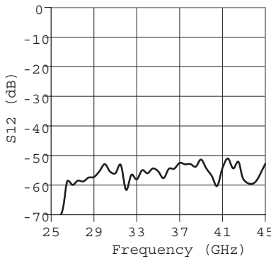
Figure 2. Typical Isolation
