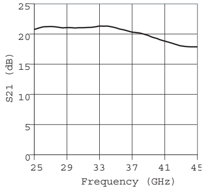
Figure 1. Typical Gain
