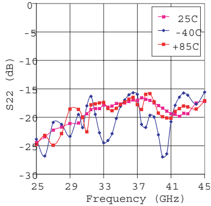
Figure 10. Output Return Loss Over Temperature
