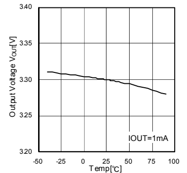
Fig. 15 Output Voltage vs Temperature (BH33NB1WHFV)
