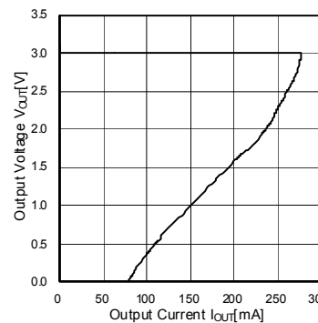
Fig. 8 Output Voltage vs Output Current (BH30NB1WHFV)
