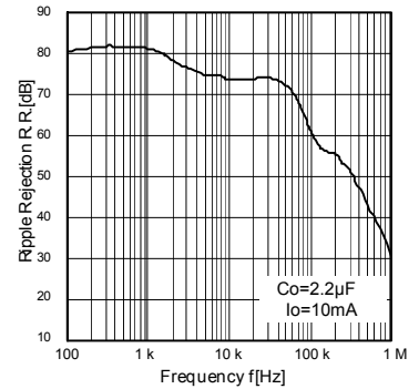
Fig. 18 Ripple Rejection (BH33NB1WHFV)
