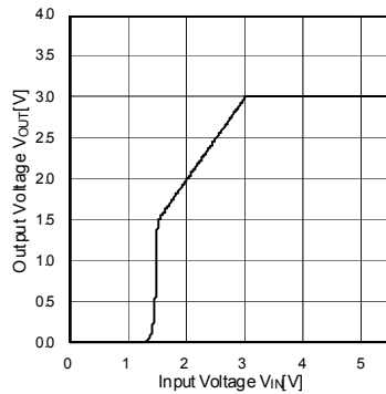
Fig. 2 Output Voltage vs Input Voltage (BH30NB1WHFV)
