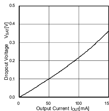
Fig. 11 Dropout voltage vs Output Current (BH30NB1WHFV)
