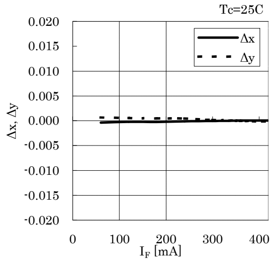
Forward Current vs. Chromaticity Coordinate
