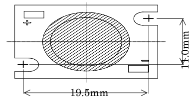
Recommended installation screw pitch
