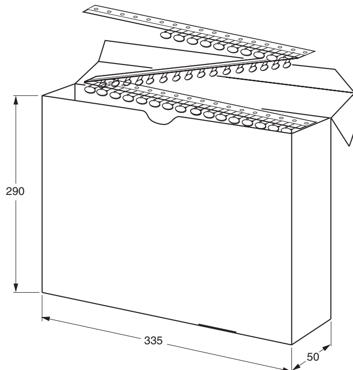
Ammopack with capacitors on tape
