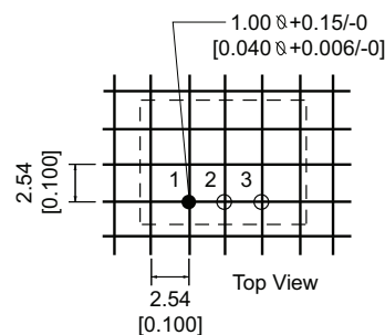
Recommended PCB Layout Pattern
