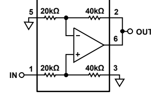
Figure 54. Noninverting Amplifier, Gain = 2
