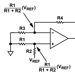
Figure 47. Ensure Sufficient Voltage Headroom on the Internal Op Amp Inputs
