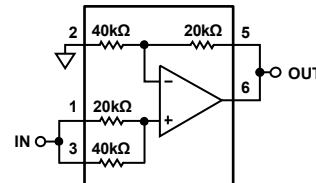
Figure 53. Noninverting Amplifier, Gain = 1.5
