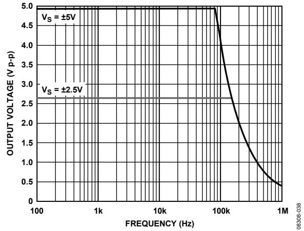
Figure 38. Maximum Output Voltage vs. Frequency, V_S = 5V, 2.7V
