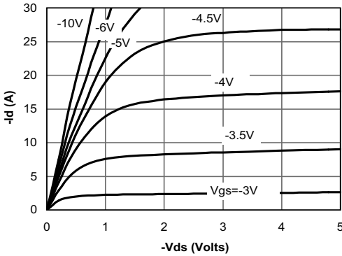
Fig 1: On-Region Characteristics
