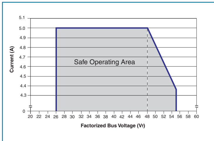
Figure 17 — PR048A480T024FP rating based on Factorized Bus voltage
