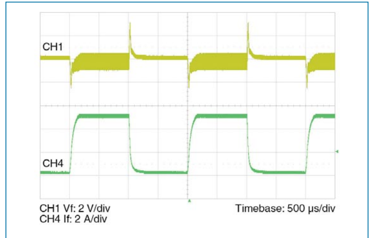
Figure 9 — Transient response; PRM alone 36 Vin, 0-5-0 A no load capacitance, local loop
