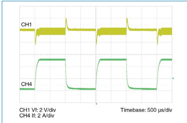
Figure 8 — Transient response; PRM alone 48 Vin, 0-5-0 A, no load capacitance, local loop
