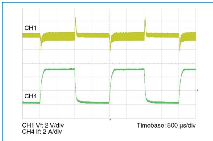
Figure 10 — Transient response; PRM alone 75 Vin, 0-5-0 A no load capacitance, local loop.
