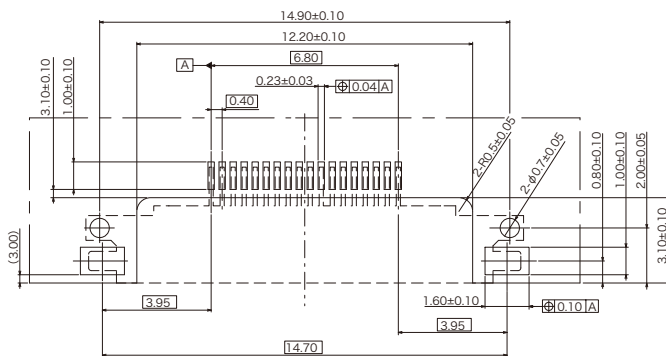
Recommended PCB Dimensions
