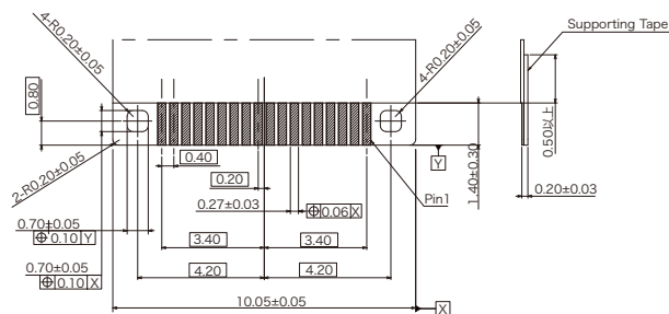
Recommended FPC Dimensions
