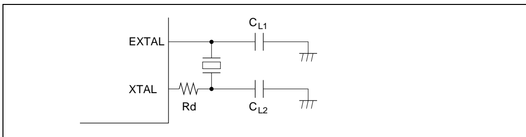
Figure 19.2 Connection of Crystal Resonator (Example)
