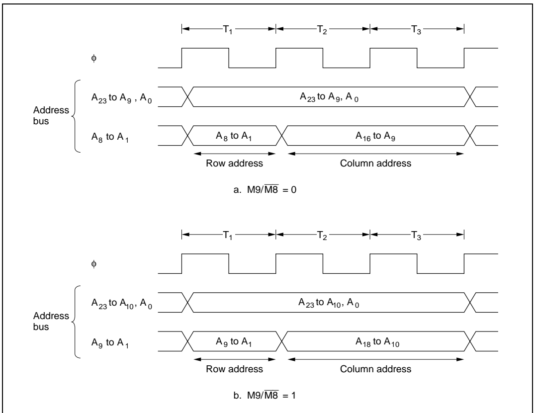
Figure 7.4 Multiplexed Address Output (Example without Wait States)
