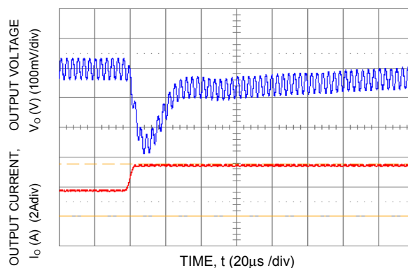
Figure 15. Transient Response to Dynamic Load Change from 50% to 100% at 28Vin, C ext - 3x10µF ceramic, C Tune =470pF & R Tune =150Ω
