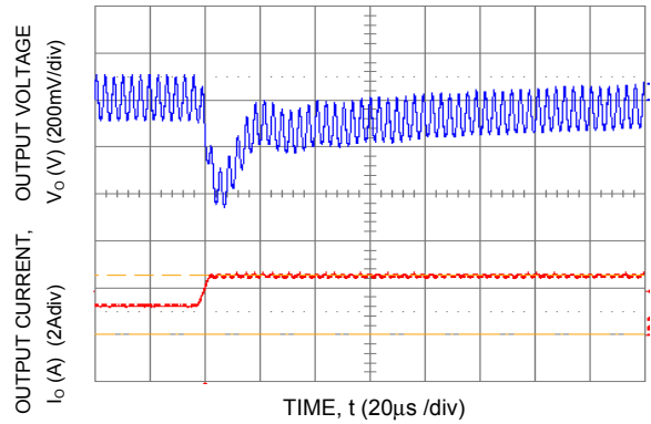
Figure 21. Transient Response to Dynamic Load Change from 50% to 100% at 28Vin, Cext - 1x10uF ceramic, CTune=150pF & RTune=220Ω
