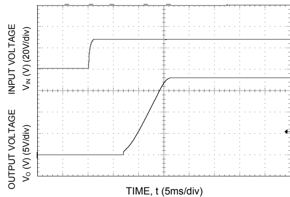
Figure 23. Typical Start-up Using Input Voltage ( V_{IN} = 28V , I_o = I_{o,max} ).
