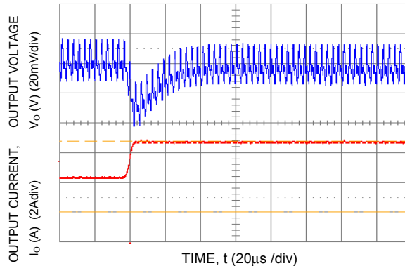
Figure 10. Transient Response to Dynamic Load Change from 50% to 100% at 28Vin, C_{ext} = 10\mu F ceramic + 330µF polymer, C_{Tune} = 10nF & R_{Tune} = 150\Omega
