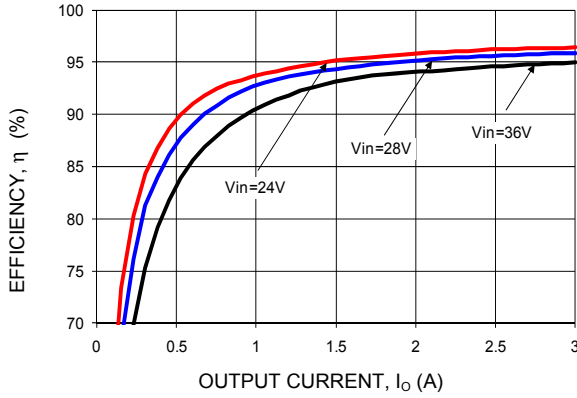
Figure 18. Converter Efficiency versus Output Current.
