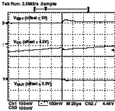
Figure 17. V_{CC} Power Up ( V_{SBR} = 5V , Load = 300mA)
