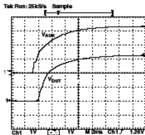
Figure 13. V_{ssv} Cold Start (Load = 400mA)
