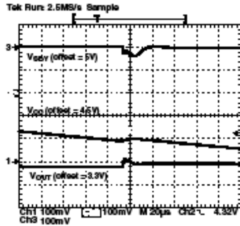
Figure 18. V_{CC} Power Down ( V_{SBR} = 5V , Load = 300mA)
