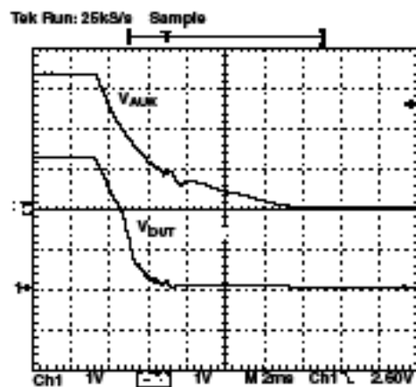
Figure 14. V_{ssv} Full Power Down (Load = 400mA)
