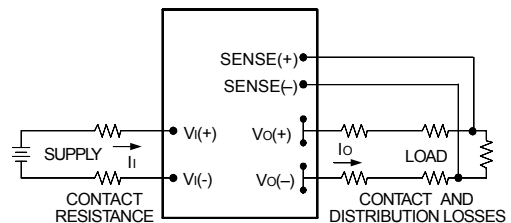
Figure 41. Circuit Configuration for remote sense .
