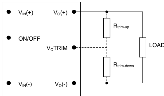
Figure 42. Circuit Configuration to Trim Output Voltage.
