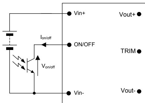
Figure 40. Remote On/Off Implementation.
