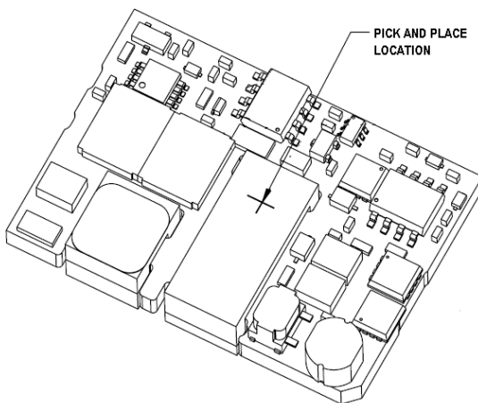
Figure 46. Pick and Place Location.
