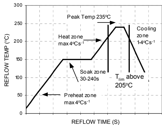
Figure 47. Reflow Profile for Tin/Lead (Sn/Pb) process
