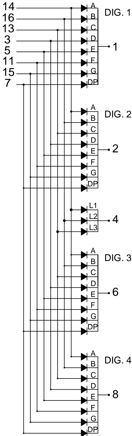
LFD4353V-XX-PF
