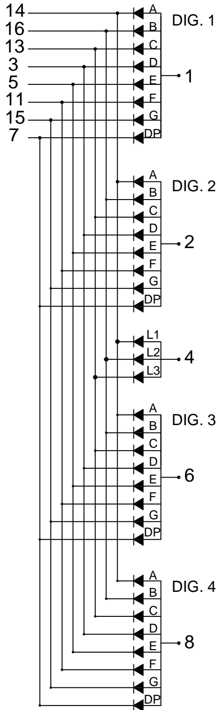
LFD4363V-XX-PF
